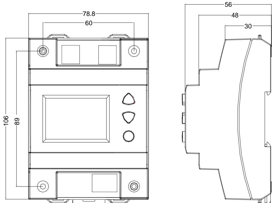
All dimensions in mm
